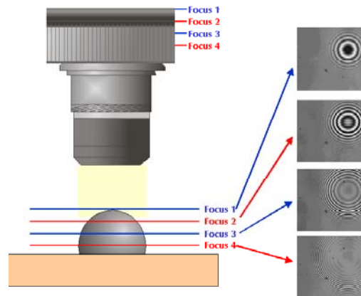
Fig. 3. Principle of vertical scanning in interferometry.
