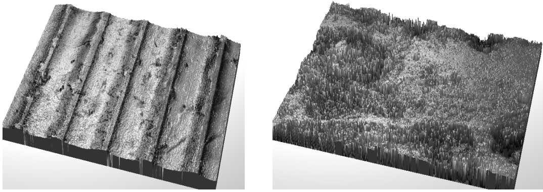
Fig. 4. Brake drum (left) and lining (right), 0 kilometres of covered distance.
