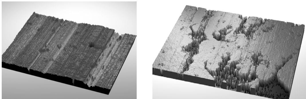
Fig. 5. Brake drum (left) and lining (right) after 250 000 kilometres of covered distance.
