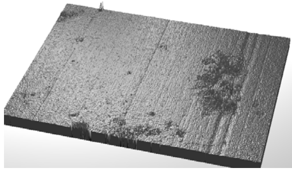
Fig. 6. Brake drum after vitrification, 80 thousands of kilometres of covered distance.
